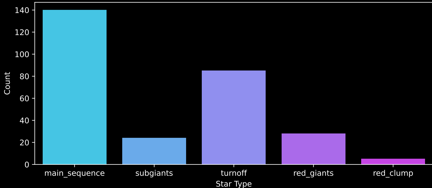
GALAH DR4 Field: [1240] Count plot of Star Type
