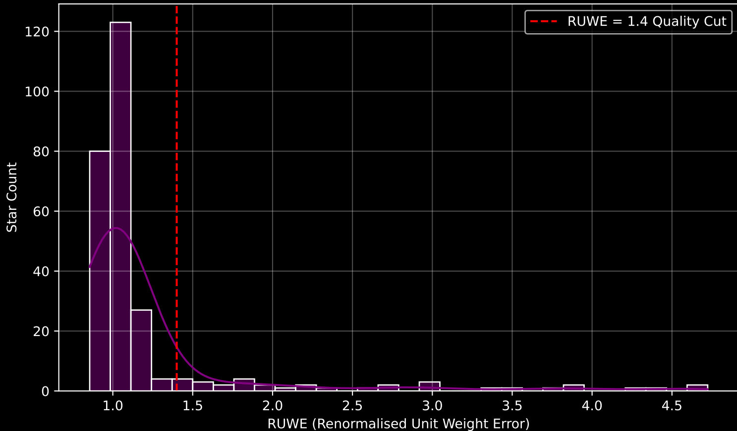
GALAH DR4 Field [1240] RUWE Distribution (n= 268)
