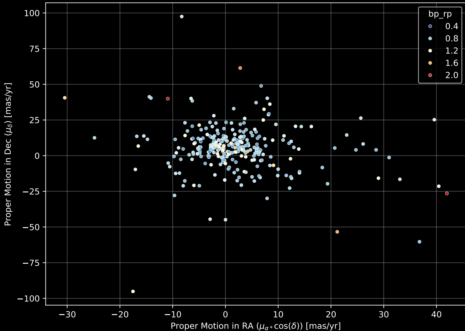
GALAH DR4 Field: [1240] Proper Motion Diagram (n= 282)
