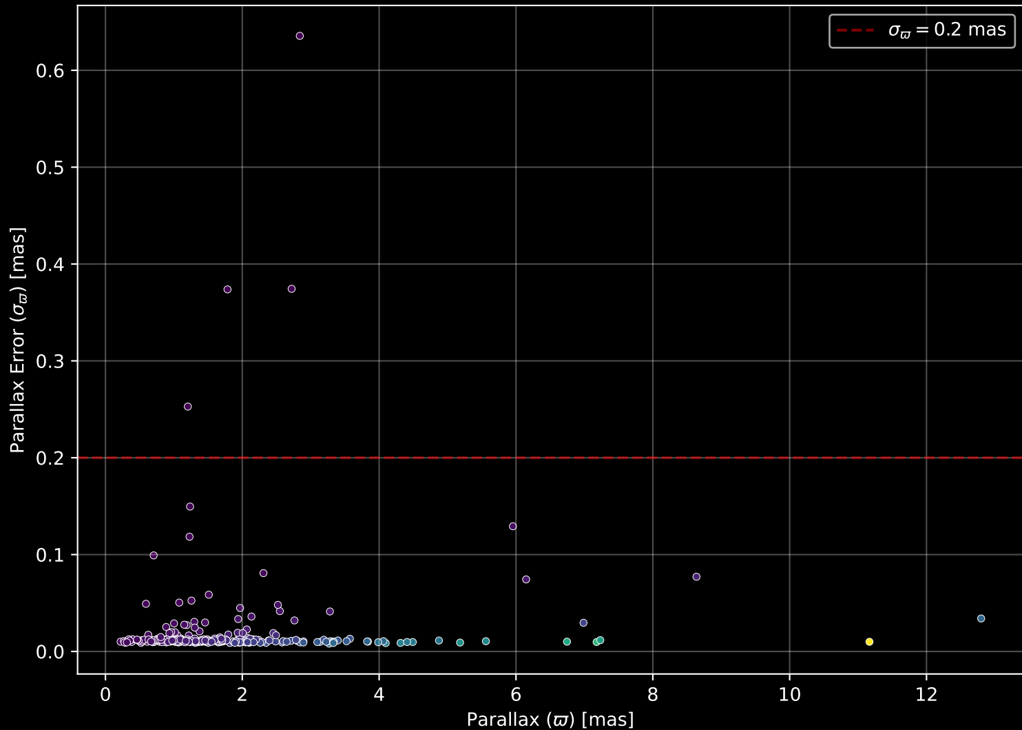
GALAH DR4 Field: [1240] Parallax Quality (n= 282)
